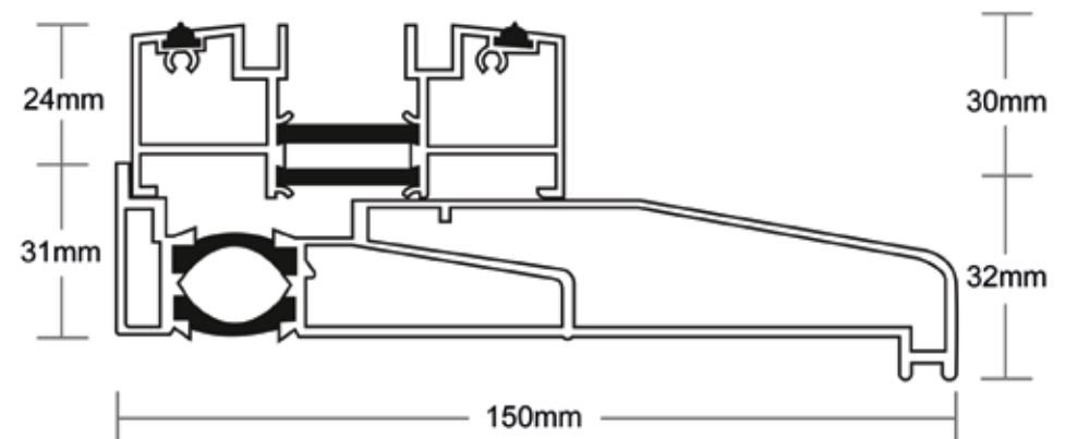
Low Threshold and Sill
