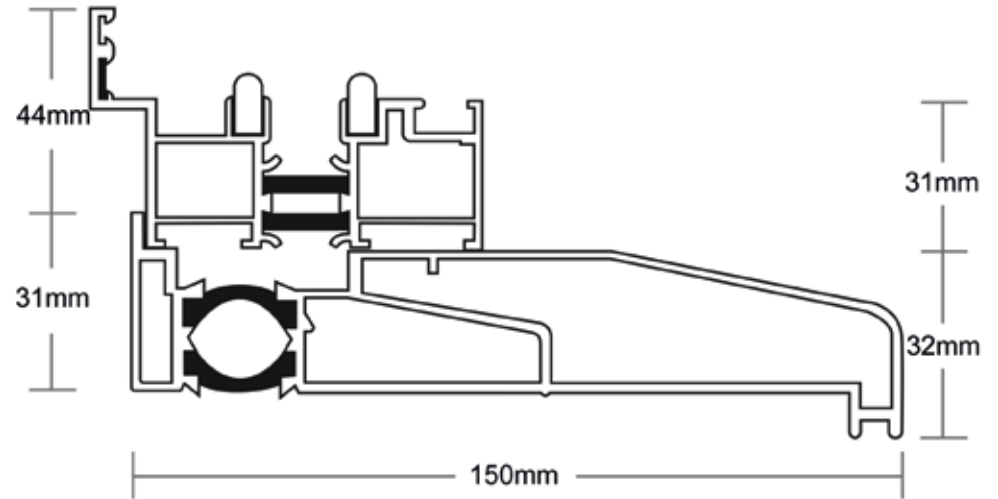
Rebated and Sill
